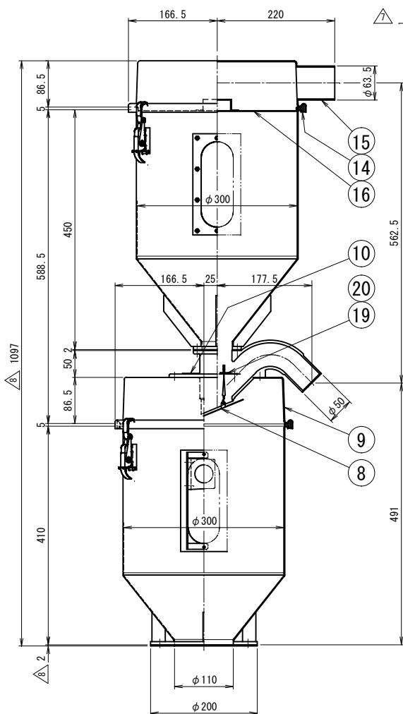
Figure from direction of A A矢視
