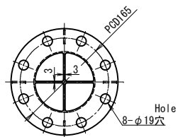
Figure from direction of A A矢視
